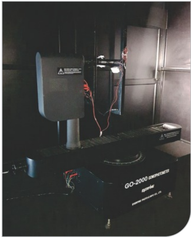
Goniophotometer
